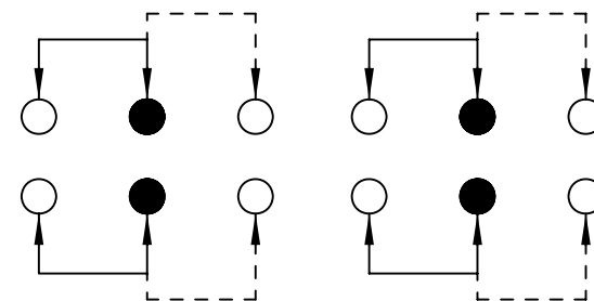
SCHEMATIC (NON-SHORTING)
